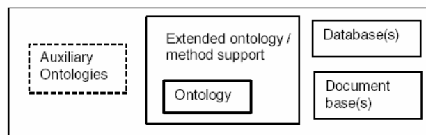
FIGURE 6: ONTOLOGY ENVIRONMENT
